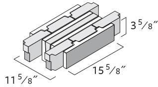
OMNI BLOCK SYSTEM 12 12" x 4" x 16"
