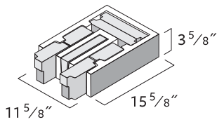
OMNI BLOCK SYSTEM 12 12" x 4" x 16"
