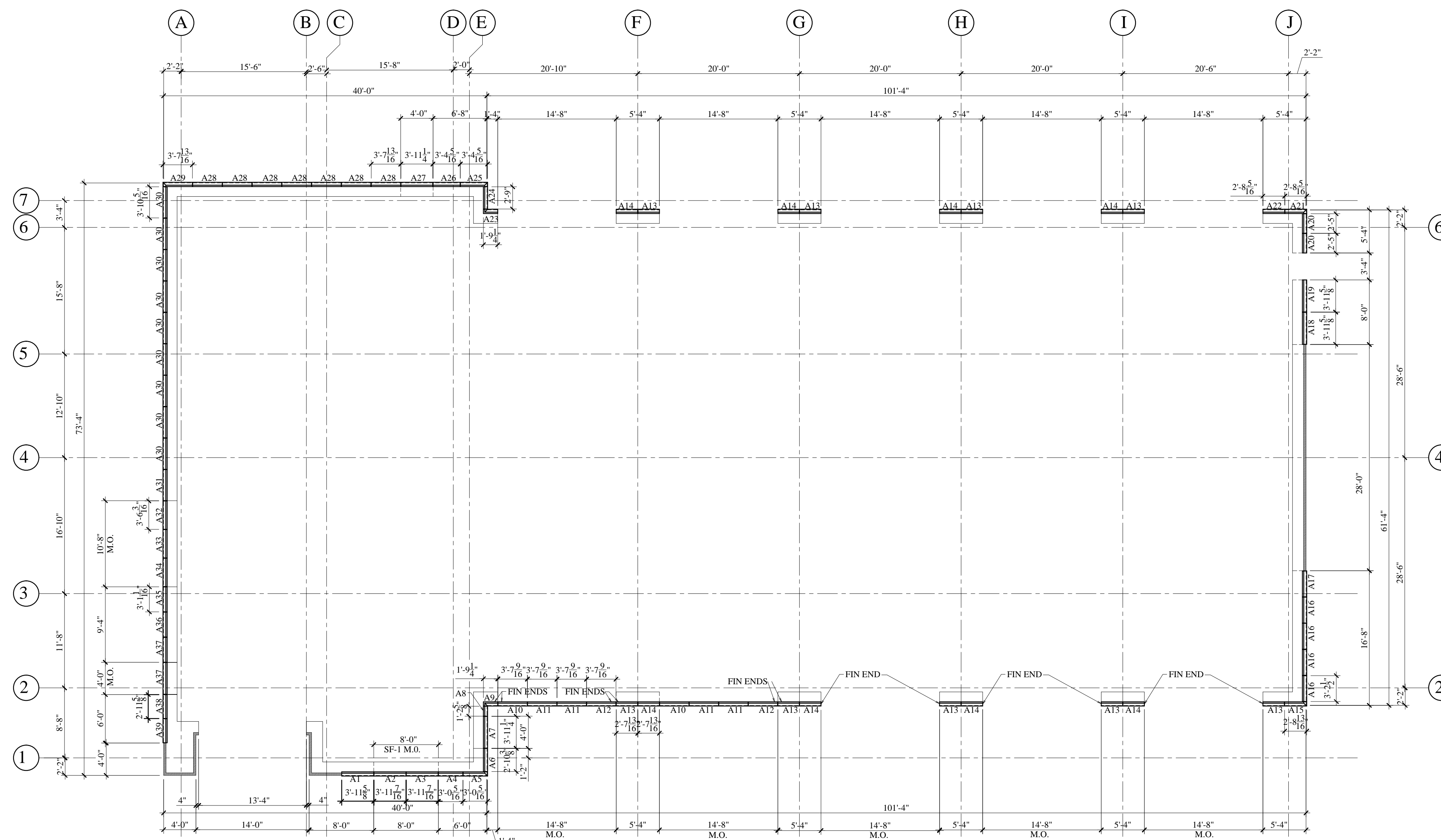
FIRS FLOOR PRECAST WATERTABLE LAYOUT ARCH REF: A11 SCALE: 1/8"=1'-0"
